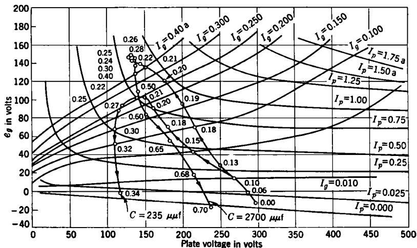
Fig. 14-26.—Operating curves for the two pulses shown in Fig. 14-25 with time intervals indicated in \mu sec.
